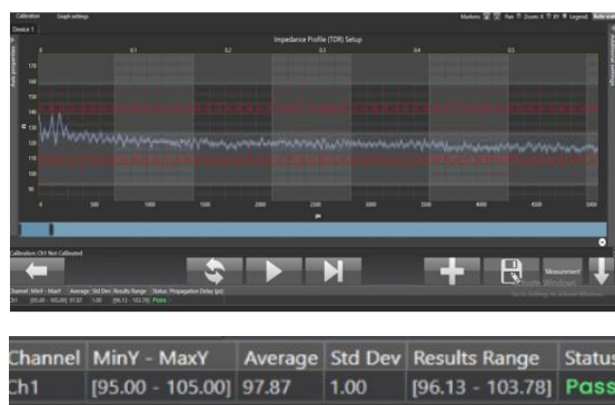
Figure 2 Impedance profile mask with pass verdict.
