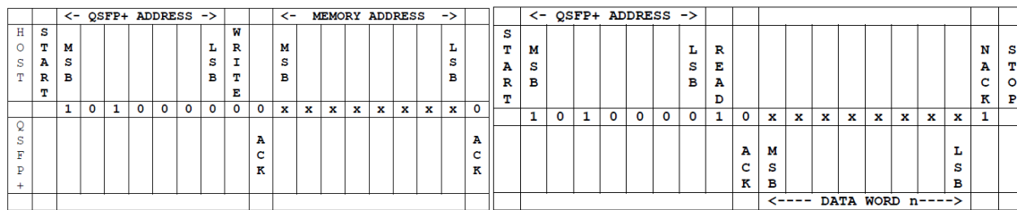
Figure 4: QSFP+ Random Read
