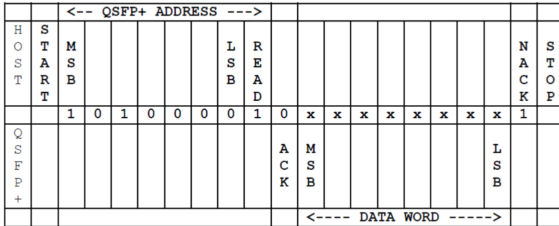
Figure 3: QSFP+ Current Address Read Operation
