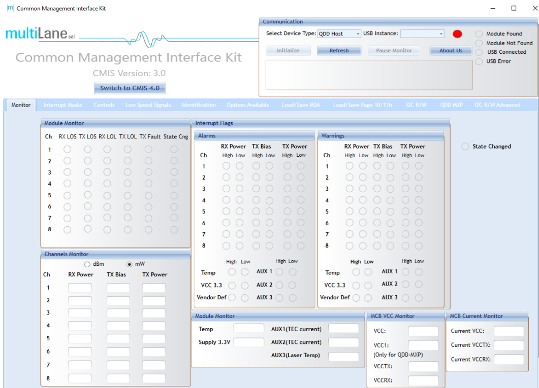
Figure 2: GUI Window
