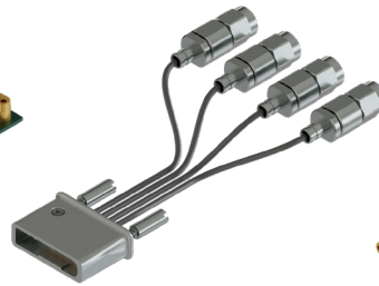
SMPS to Precision RF Coax Cable Assembly
