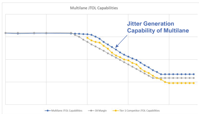
MultiLane JTOL Performance
