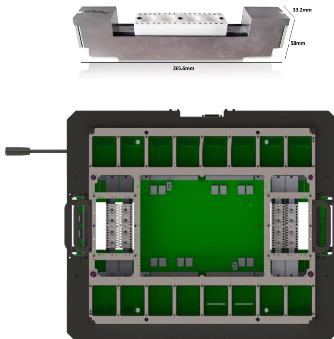
Figure 1: Four ML cassettes mounted in an Advantest V93K HSIO test head extender frame
