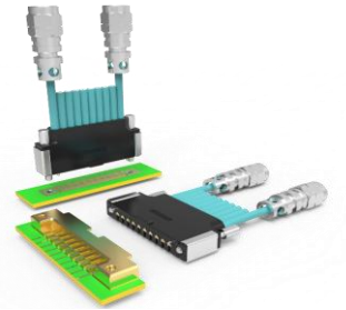
Figure 3: 8 channel coreHC to 1.85mm cable
