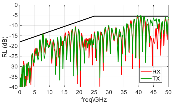
Figure 5: Return Loss – IEEE P802.3ck-D3.0
