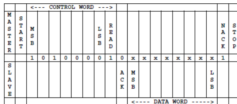
Figure 2: OSFP Current Address Read Operation
