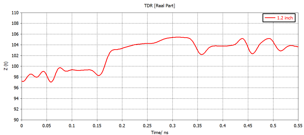
Figure 5: Impedance profile 1.2 inch channel
