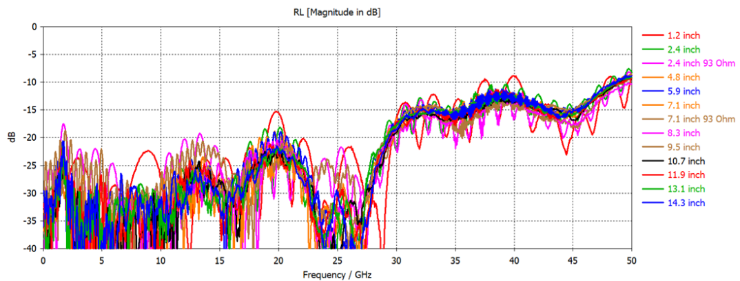
Figure 4: Return loss
