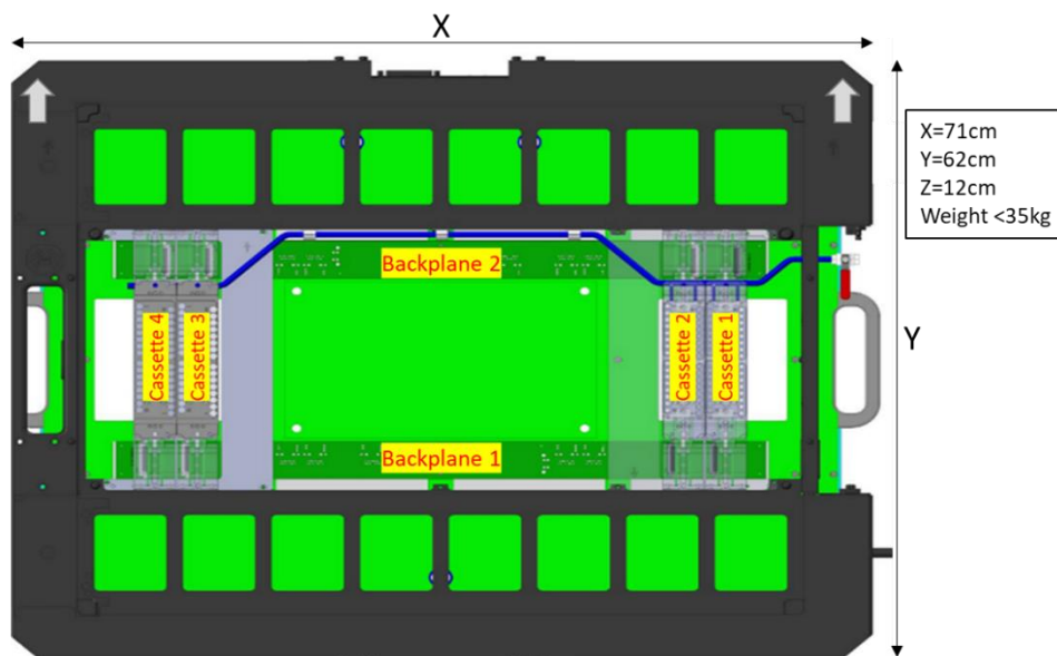
Twinning Frame Rendition showing installed instruments and backplane
