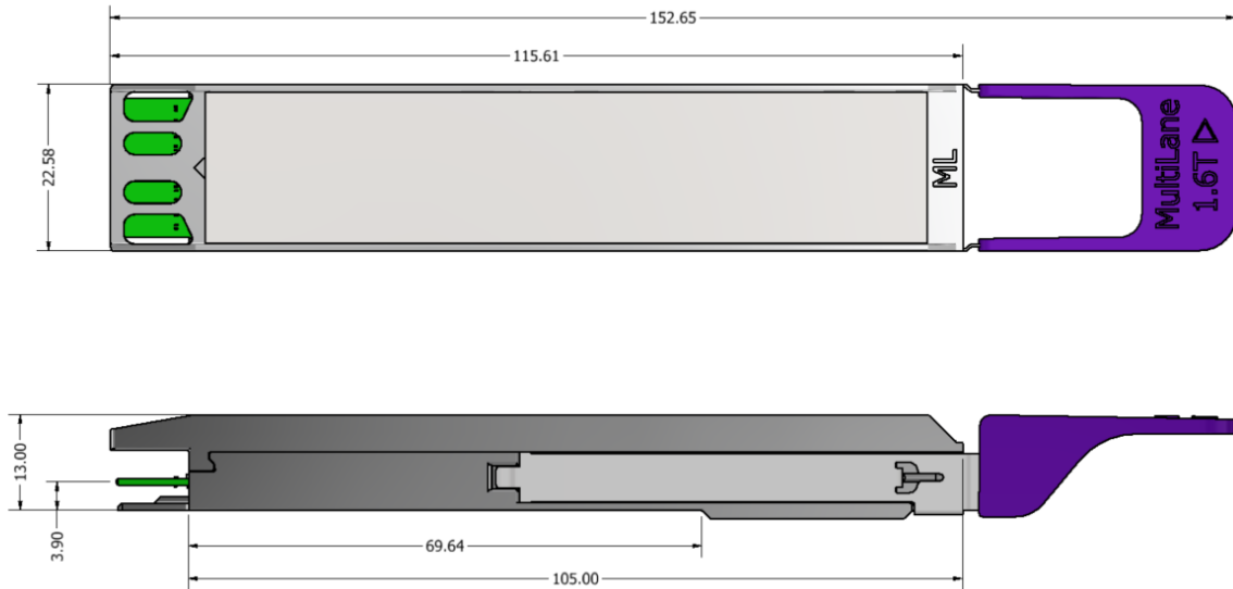
Figure 11: ML4064-AL6I-224 Mechanical Dimensions
