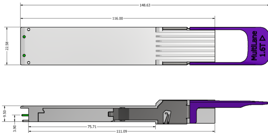
Figure 12: ML4064-AL6R-224 Mechanical Dimensions
