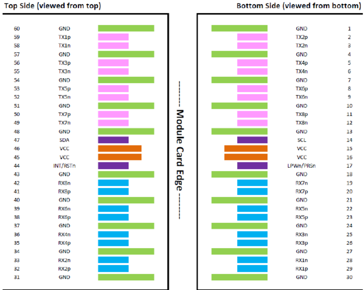
Figure 10: OSFP Module Pad Layout
